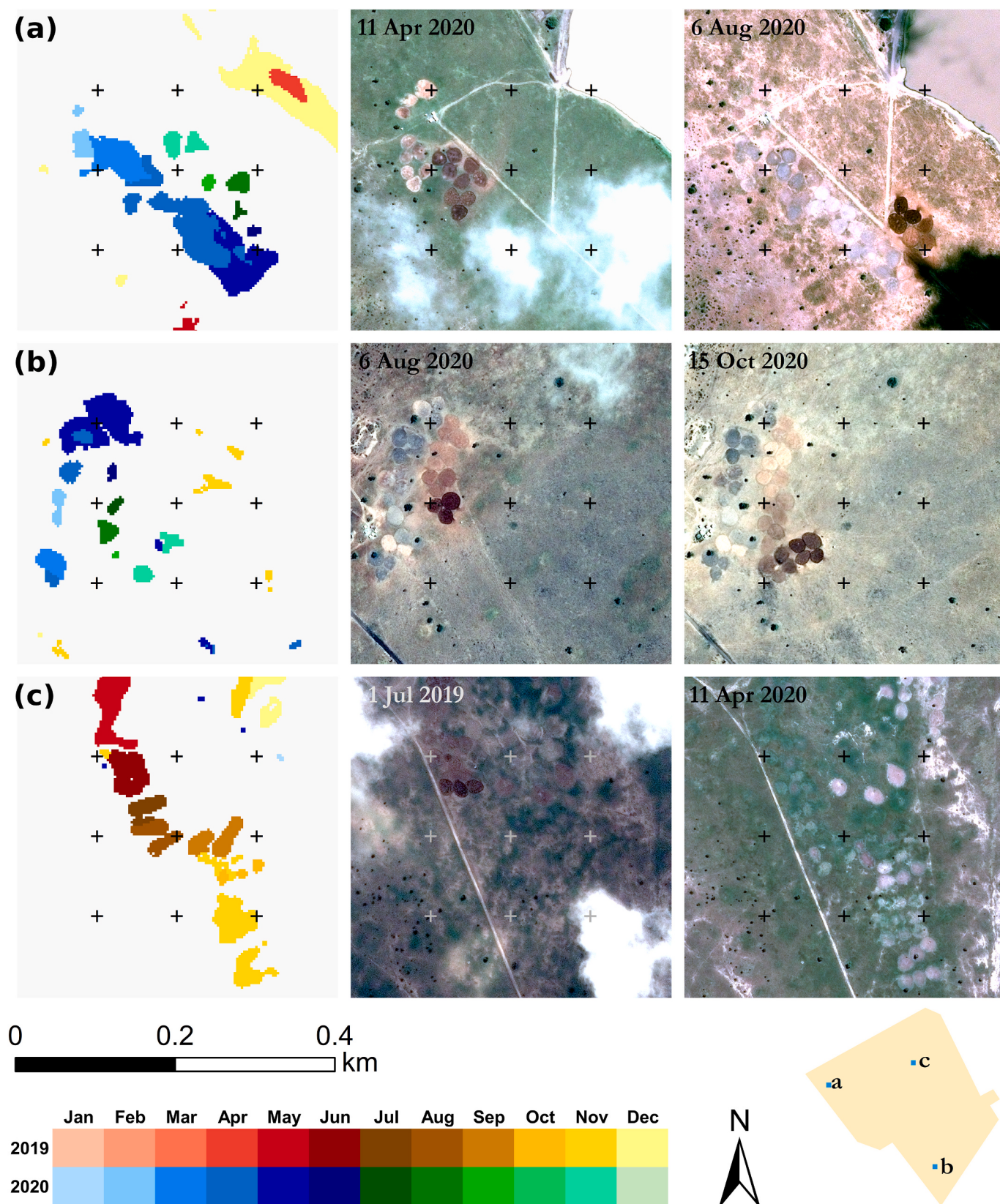
Fig. 13. Detailed view of start dates of PlanetScope-retrieved bomas for three subsets. The crosses are added for better visual comparison and are placed every 100 m. The location and extent of each subset within Kapiti is indicated with blue squares on the bottom right inset. For each subset two Pleiades images are shown. The top right area of (a) corresponds to surface water behind a dam. (For interpretation of the references to colour in this figure legend, the reader is referred to the web version of this article.)
