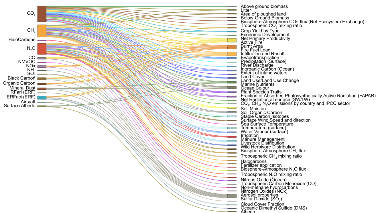
Fig. 2 On the left, climate forcing components as defined in the IPCC Fifth Assessment Report (Myhre et al. 2013) and on the right, the environmental variables found to be essential to quantify these components for the African continent
